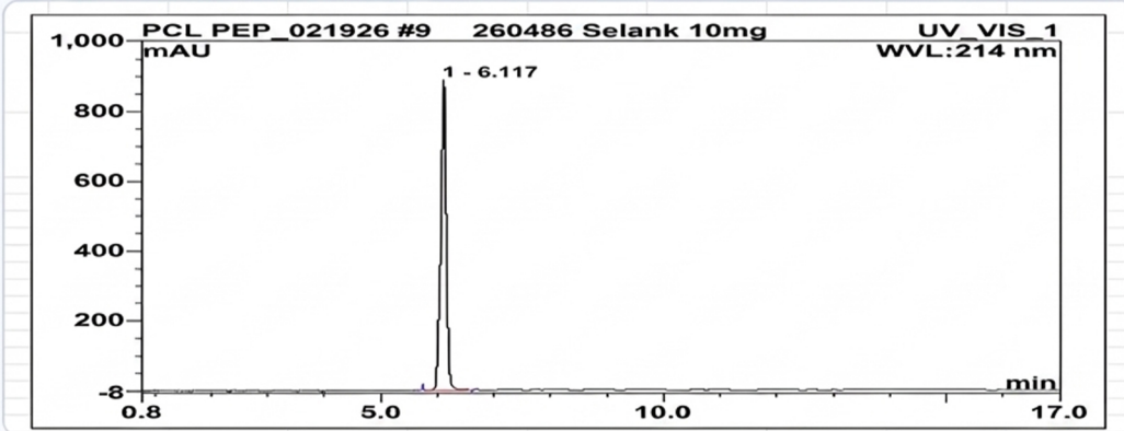
HPLC Chromatogram (Retention Time: 6.117 min)
